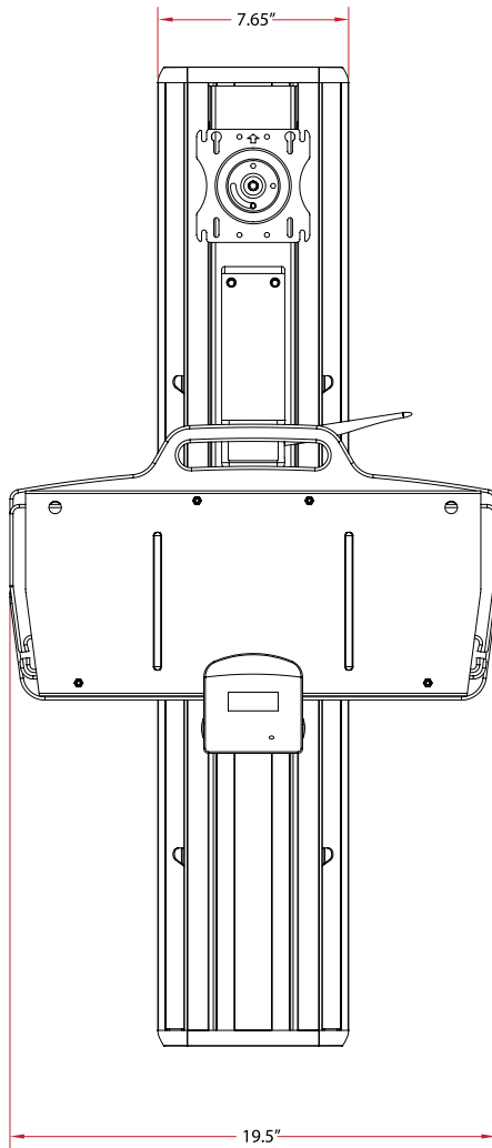
HWM48S - Hover WM Slim Workstation
